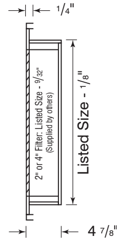
RRF4 for 2" or 4" filter
