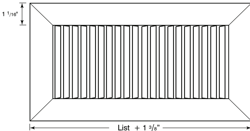
REAL Residential Floor Bar Grille
