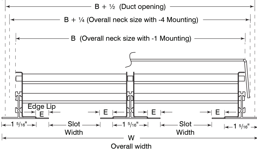
ALF20 without pattern-control damper
